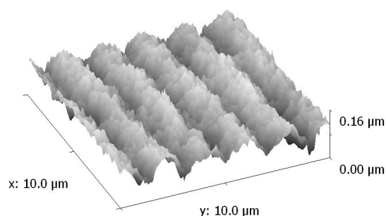
Fig. 3. AFM picture of the surface diffraction grating created by holographic recording at 325 nm.
