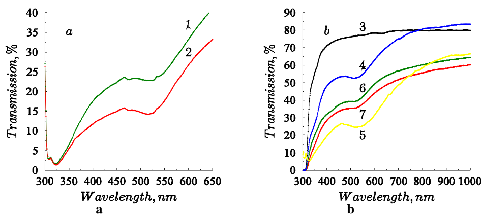
Fig. 1. Optical transmission spectra : (a) - for 10 wt % SiO 2 - 0,3 wt% AuNPs-AmAc nanocomposite (1- monomer, 2-polymer); (b) - for SiO 2 -0,2 wt% AuNPs-UDMA nanocomposites: (3) - 10 wt% SiO 2 /UDMA polymer; (4) 26wt% SiO 2 / 0.2 wt% AuNPs/ UDMA, monomer; (5) - 26wt% SiO 2 / 0.2wt% AuNPs/ UDMA, polymer; (6) - 10wt% SiO 2 / 0.2wt% AuNPs/ UDMA, monomer; (7) -10wt% SiO 2 / 0.2wt% AuNP/ UDMA, polymer
