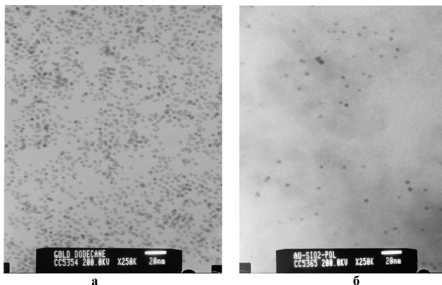
Fig. 2. TEM pictures of AuNPs in different matrix: Material – a) UDMA/ 0,2 wt% AuNPs/ 10% SiO 2 NPs; b) 0,2 wt% Au NP/UDMA with SiO 2
